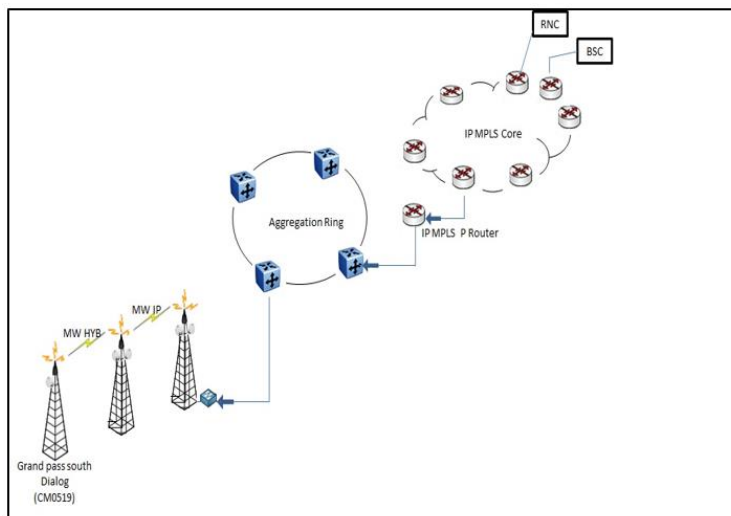
Figure 3.1: New Transport Network Architecture
